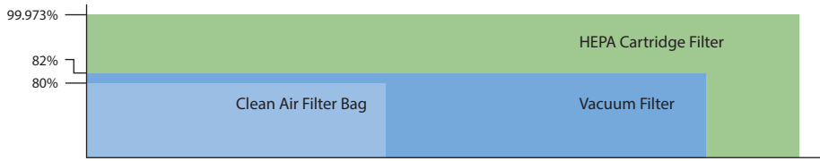
Canister Vacuum Filtration Efficacy at 0.3 Microns
